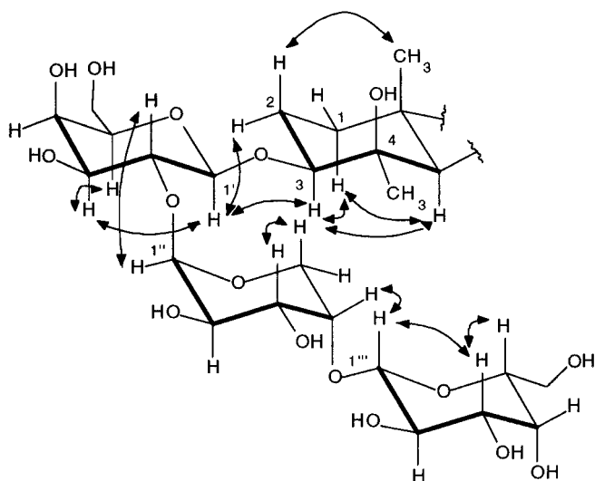
Figure 1. Key ROESY correlation peaks detected for compound 1
